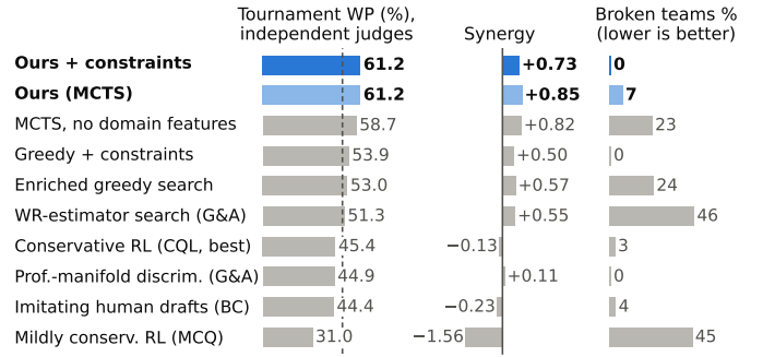
Fig. 1. Results at a glance: the eleven-strategy round-robin (110 ordered pairs \times 200 drafts; Section VII-A). First column: mean win probability under four composition-corrected judges that share no data with any agent (dashed line: 50%); the CQL row shows the better variant per column. Anchoring to human behavior is safe but blind to interactions; greedy value search sees interactions but is unsafe; MCTS reaches both, and constraint masking removes its residual broken teams with a small gain in win probability.
